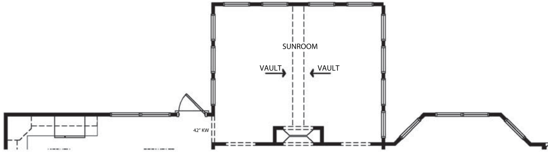
SUNROOM OPTION
