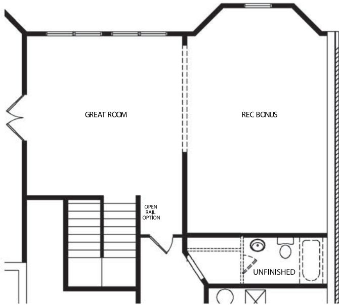
DOUBLE BASEMENT BONUS OPTION
