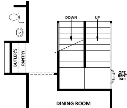
OPEN STAIRS OPTION
